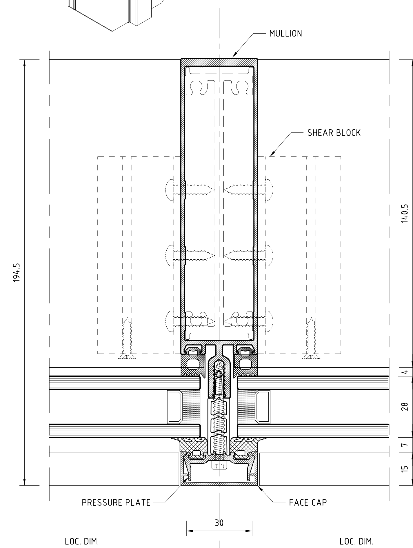
TYPICAL MULLION DETAIL
